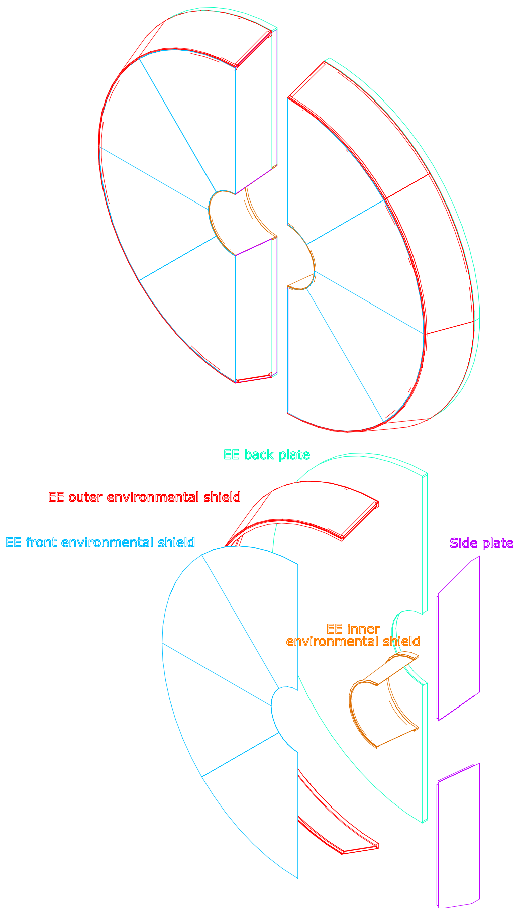
Figure 3.5.2 Component parts of the EE environmental shield.
