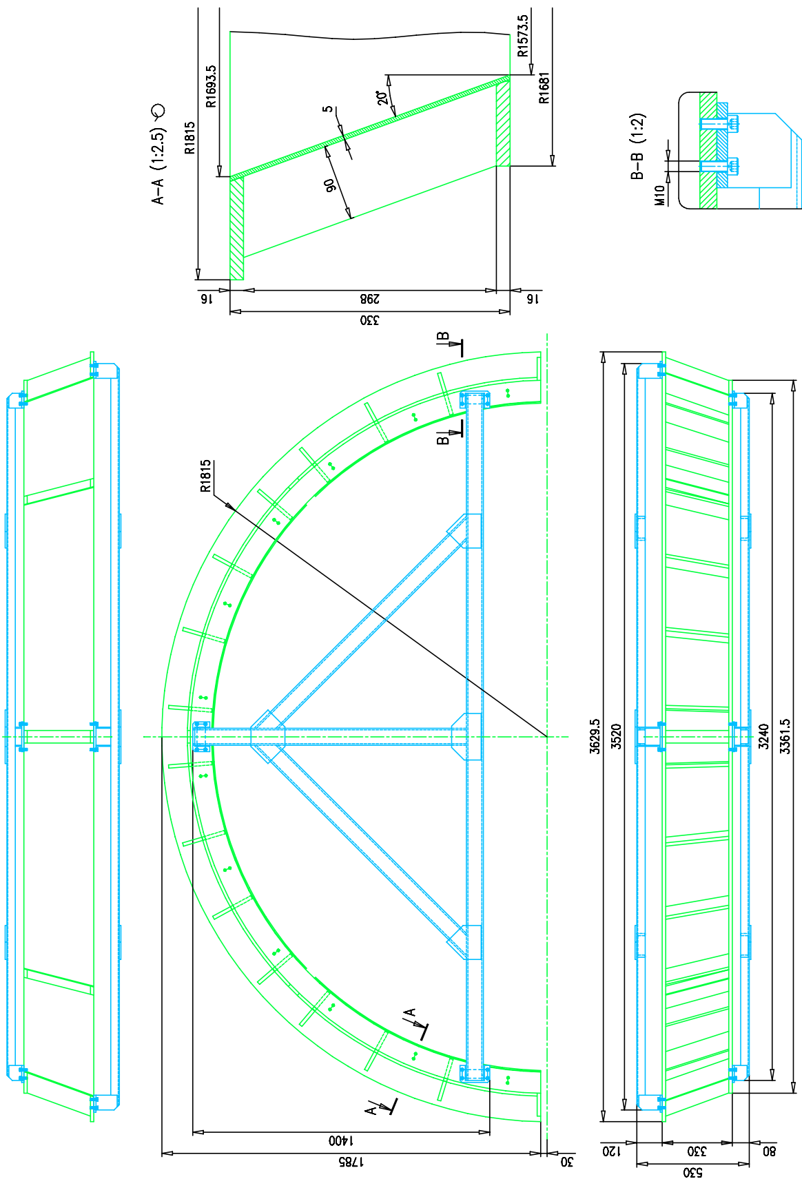
Figure 3.5.10 Tooling design for the EE environmental shield assembly and installation.
