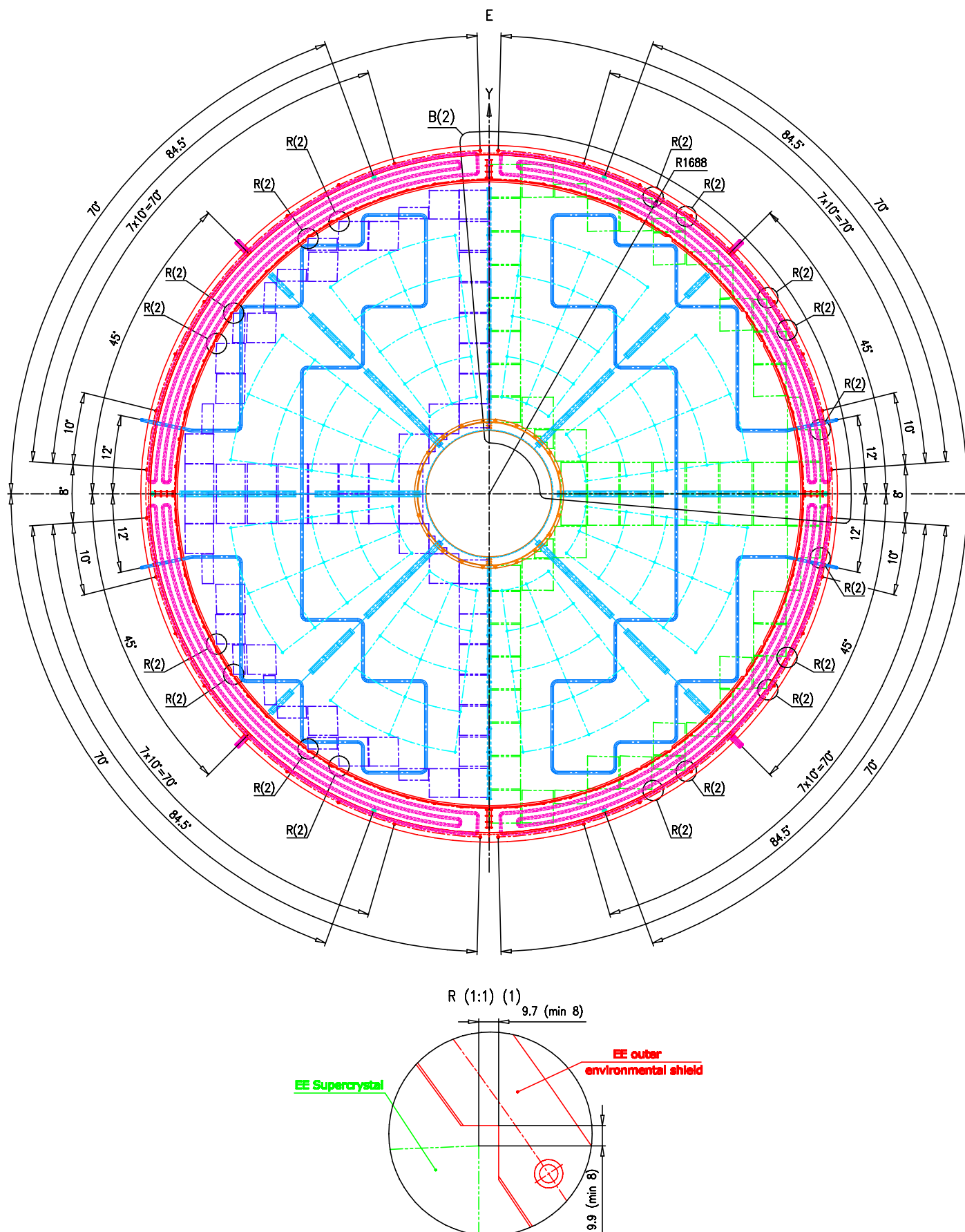
Figure 3.5.4 EE environmental shield design (back view).
