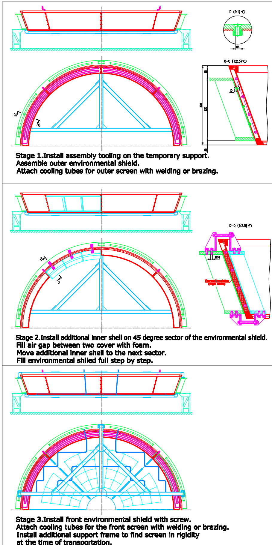
Figure 3.5.11 Technology of the EE environmental shield assembly.
