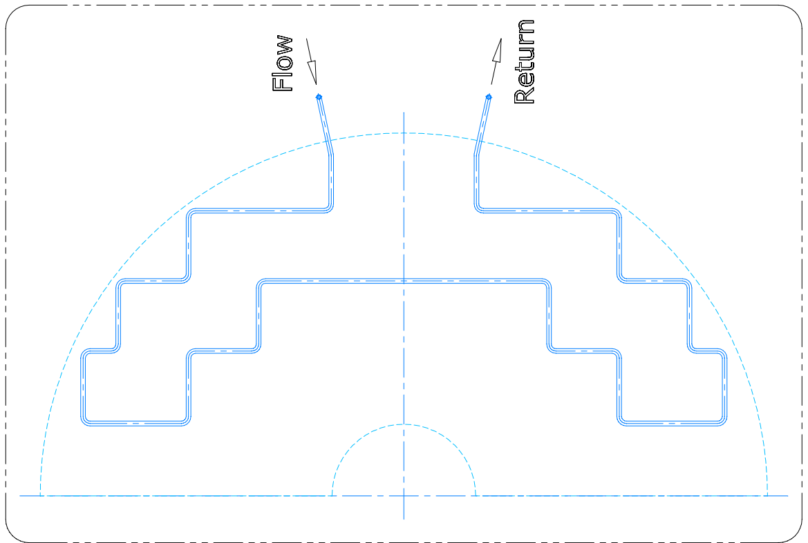
Front environmental shield (X1 per Dee)
