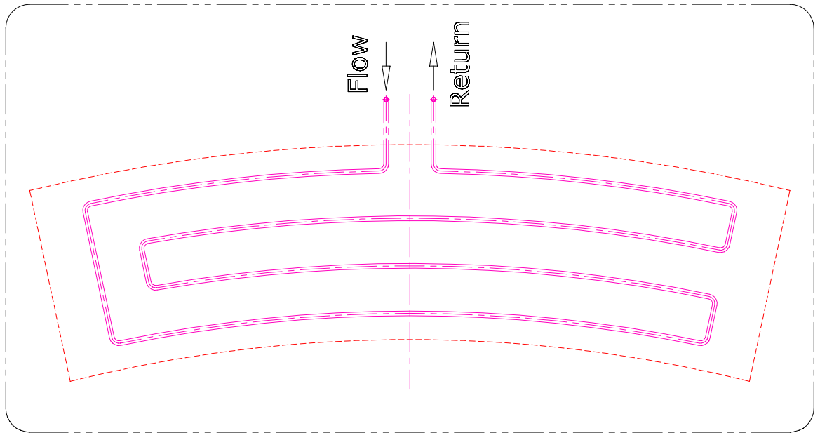
Outer environmental shield (X2 per Dee)
