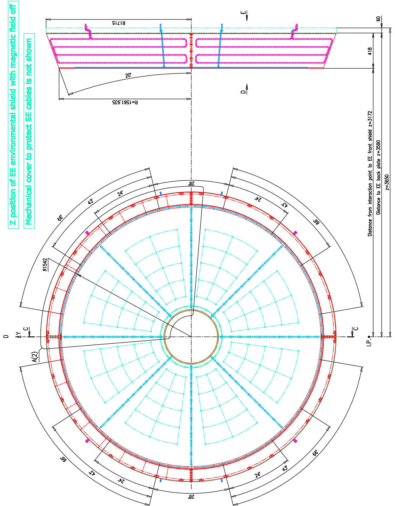
Figure 3.5.3 EE environmental shield design (front and side view).
