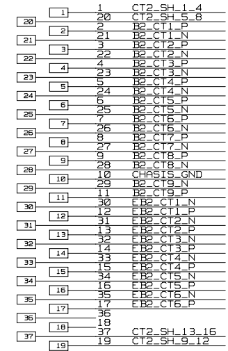
CALORIMETER_TRIGGER CABLE_2 (CT2) SK-DIN41612-37 DSUB RT-ANG
