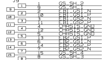
SK-DIN41612-15 DSUB RT-ANG
