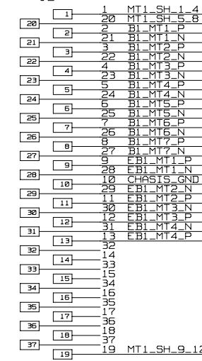
MUON_TRIGGER CABLE_1 (MT1) SK-DIN41612-37 DSUB RT-ANG
