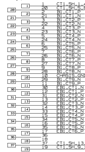
CALORIMETER_TRIGGER CABLE_1 (CT1) SK-DIN41612-37 DSUB RT-ANG
