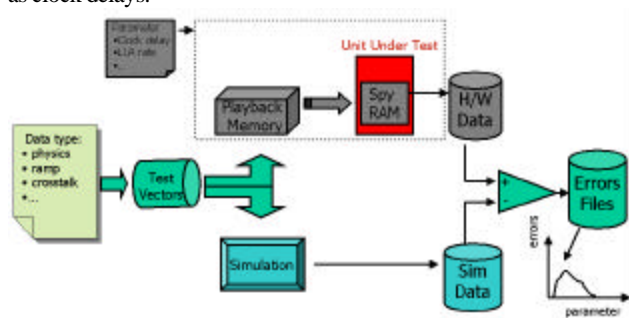
Figure 3: Schematic of the test procedure
