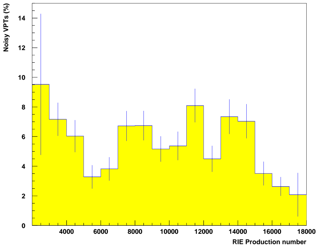
Figure 1. Fraction of noisy tubes as a function of RIE production number. Only VPTs with bar-codes in the range 1501-10000 are included.
