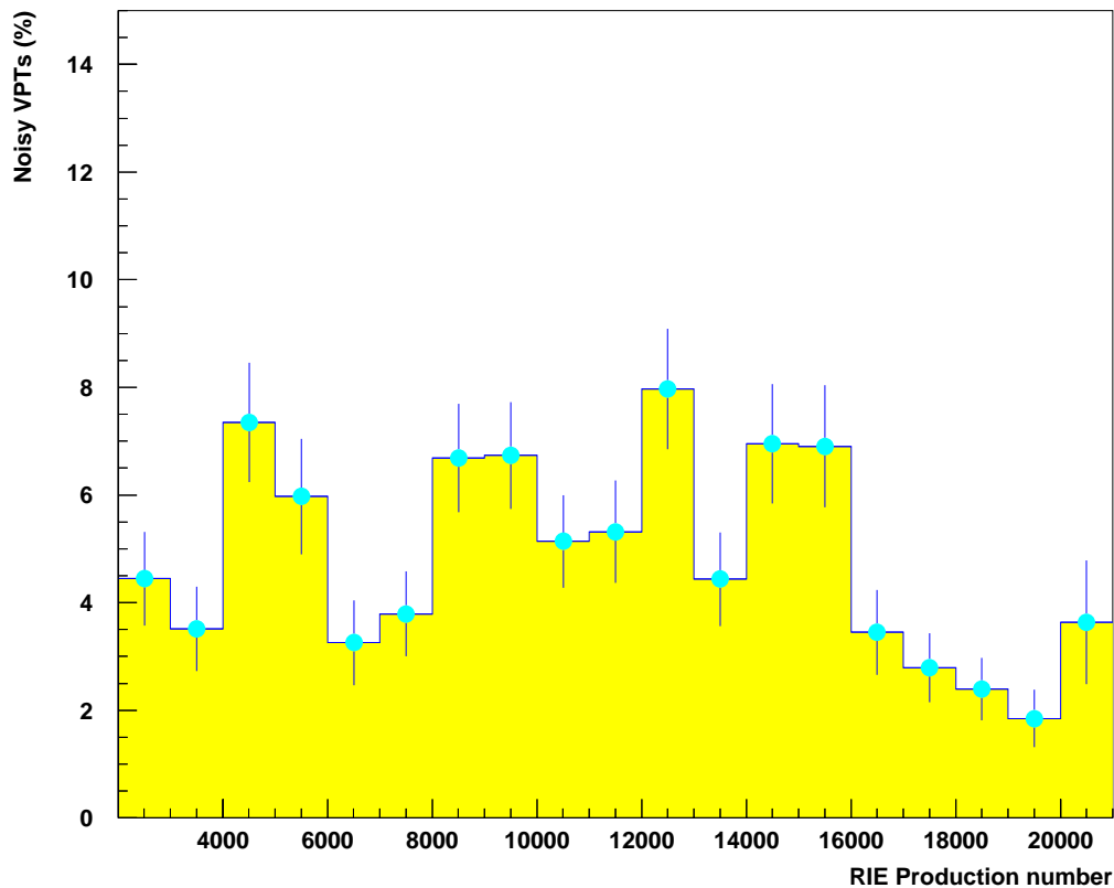
Figure 1. Fraction of noisy tubes as a function of RIE production number. Only VPTs with bar-codes in the range 501-11600 are included.
