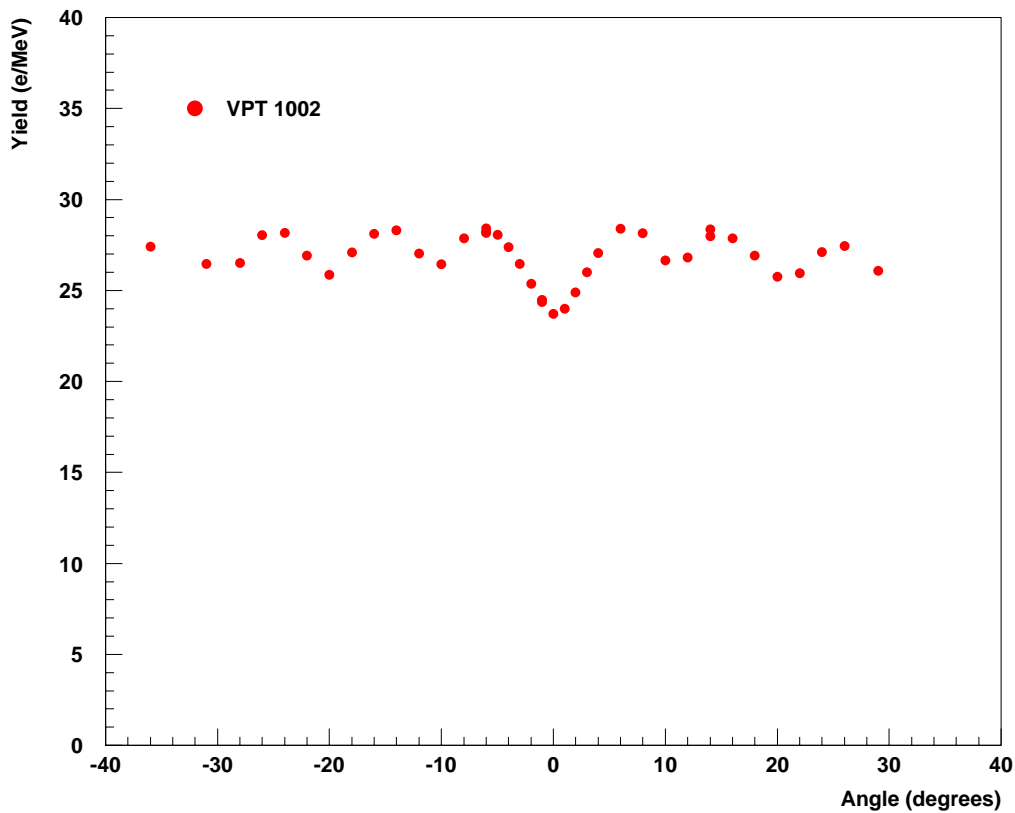
Figure 4. Angular scan at 1.8T on a typical VPT
