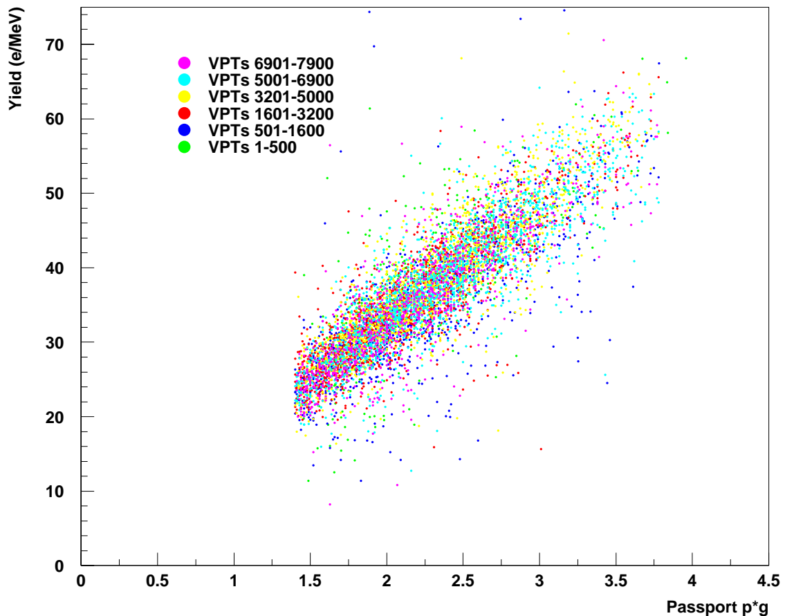
Figure 6. VPT response at 8°-25° and 1.8T v quality factor PG
