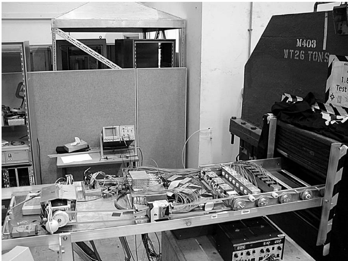
Figure 2. General view of the RAL test rig
