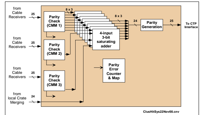
Figure 4: The system-merging logic of the e/\gamma System-level CMM.
