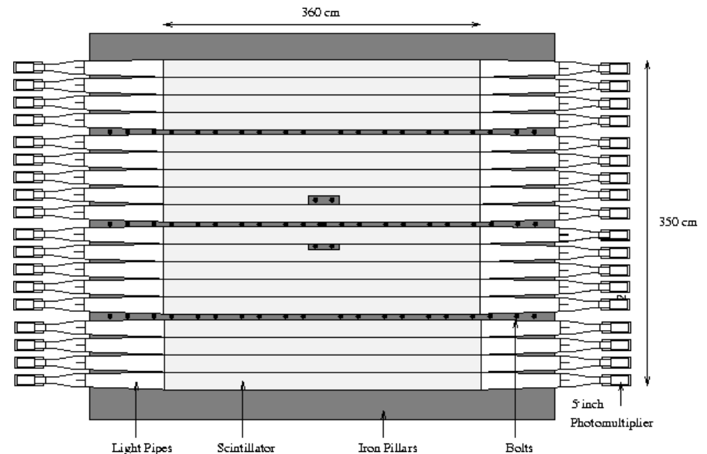
Hadronic Calorimeter from NOMAD experiment
